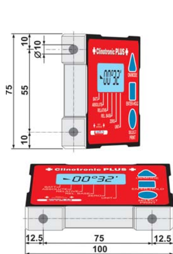
Left picture: +CLINO PLUS+ with magnetic inserts left and bottom / e.g. 015-PLUS-FG45 Right picture: +CLINO PLUS+ threaded holes M3 left and bottom / e.g. 015-PLUS-LG45
