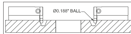
Measuring contacts for face-groove and V-groove \phi measurement
