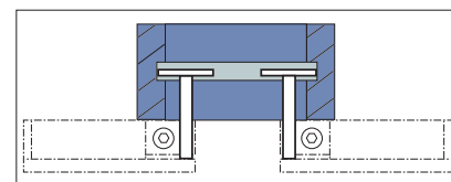
Disc anvils Code: TGUA 013
