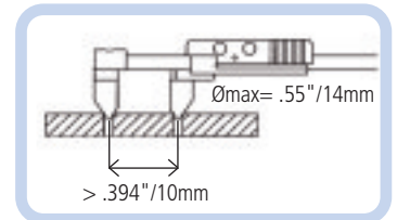
External & Internal Grooves
