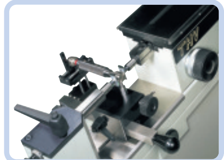
3) Checking of plug gauges and thread plug gauges
