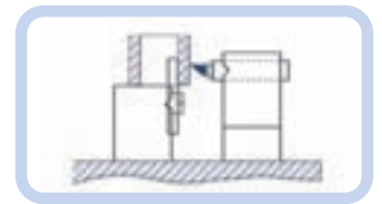
Concentricity/wall thickness
