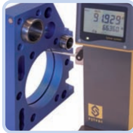
Internal diameter measurement
